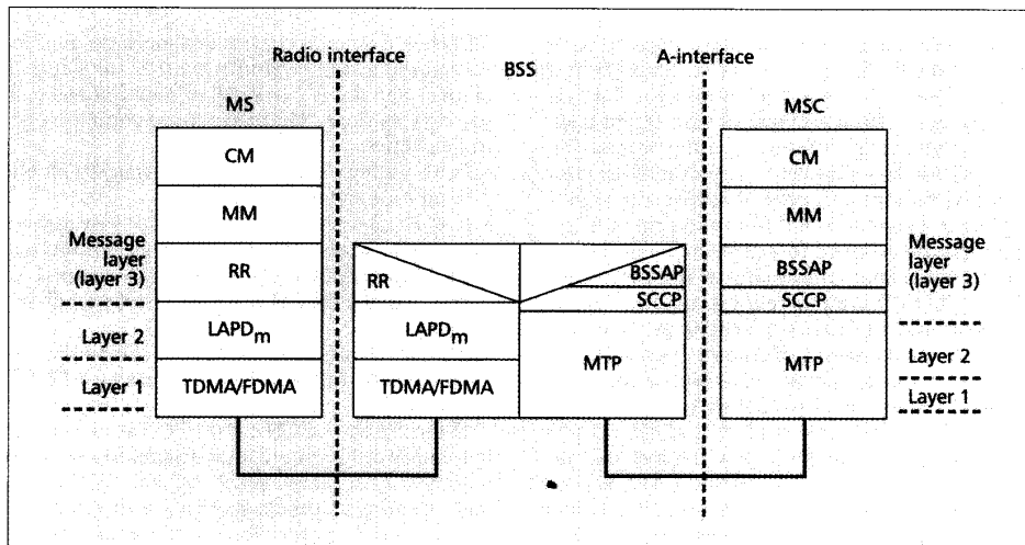
■ Figure 3. GSM protocol architecture.
